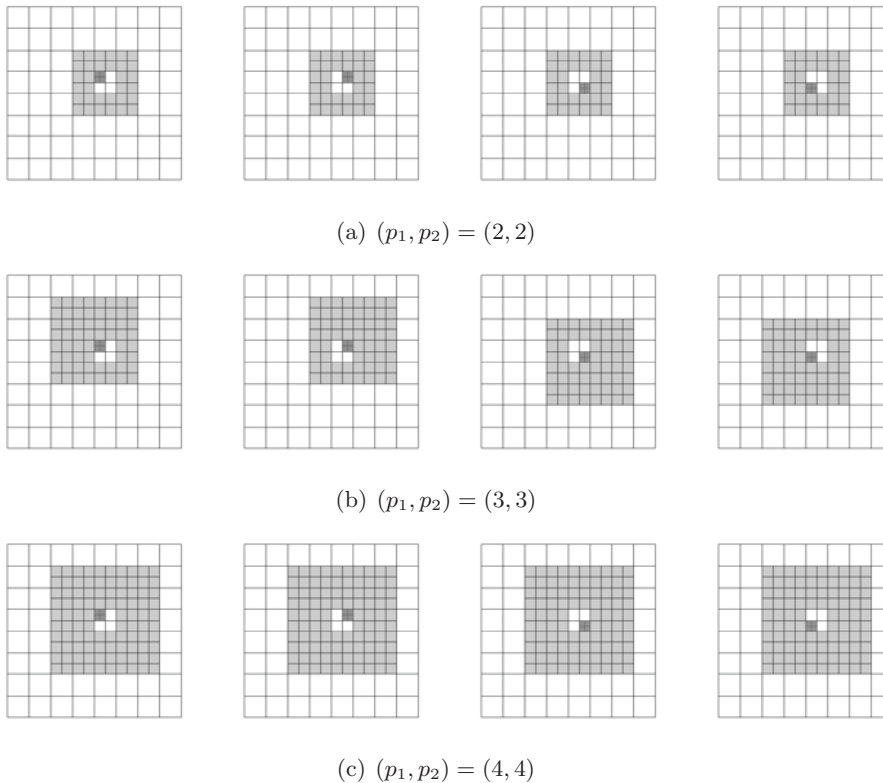
Figure 2: Neighborhood \mathcal{N}(Q, Q, 2) (light gray) of an element Q (represented by any of the four cells in dark grey) when dyadic refinement is considered for some low degree cases. Note that the neighborhood is always aligned with the grid lines of a previous hierarchical level.
