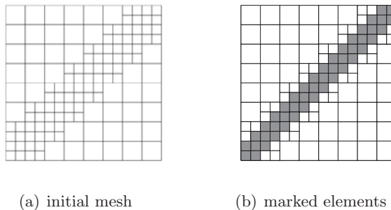
Figure 4: The admissible meshes in Fig. 1 related to the cases (p_1, p_2) = (i, i) for i = 2, 3, 4 are generated by the call to \mathcal{Q}^* = \text{REFINE}(\mathcal{Q}, \mathcal{M}, 2) to the mesh \mathcal{Q} depicted in (a) with the marked set \mathcal{M} of elements shown in (b).
