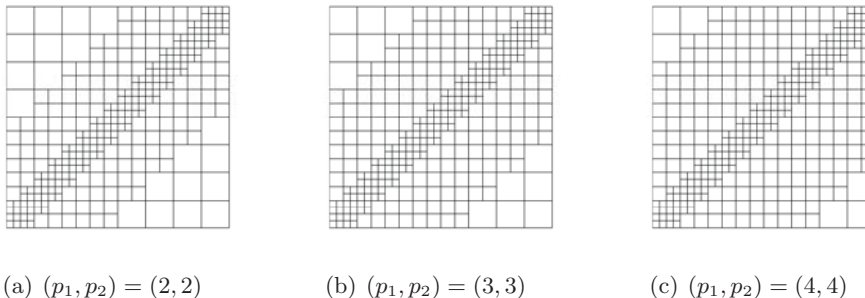
Figure 1: Admissible meshes of class 2 considered in Example 8 with respect to different degrees.
