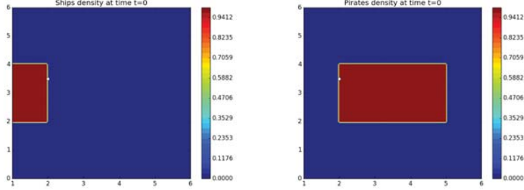
FIGURE 1. The initial densities A_0 (left) and \rho_0 (right) for the simulation of Subsection 4.1.
