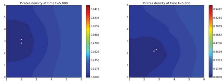
FIGURE 4. The density at the final time T = 5 for the pirates with M = 2 police watercrafts. On the left, the case of one control pointing to the north and one to the south. On the right, the case of one control pointing to the south and one to the east.
