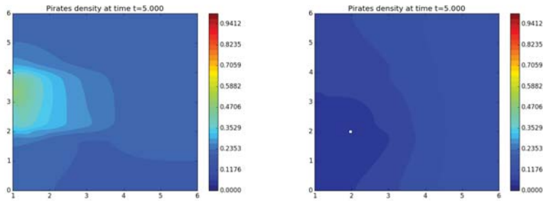
FIGURE 3. The density at the final time T = 5 for the pirates. On the left the case of M = 0 police watercrafts. On the right the case of M = 1 police watercraft.
