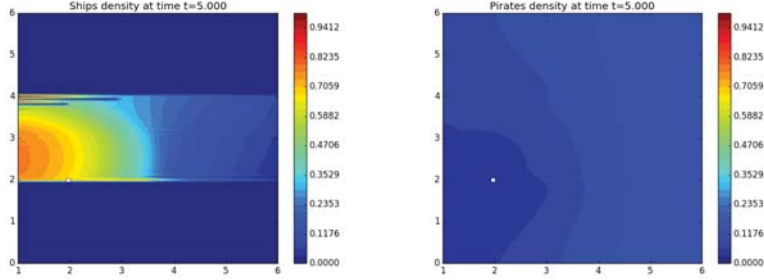
FIGURE 2. The densities at the final time T = 5 for the commercial cargos (left) and for the pirates (right). Note that around the position of the police watercraft (the white point) the pirate density is low. Moreover the cargo ships adjust their positions according to the one of the police.
